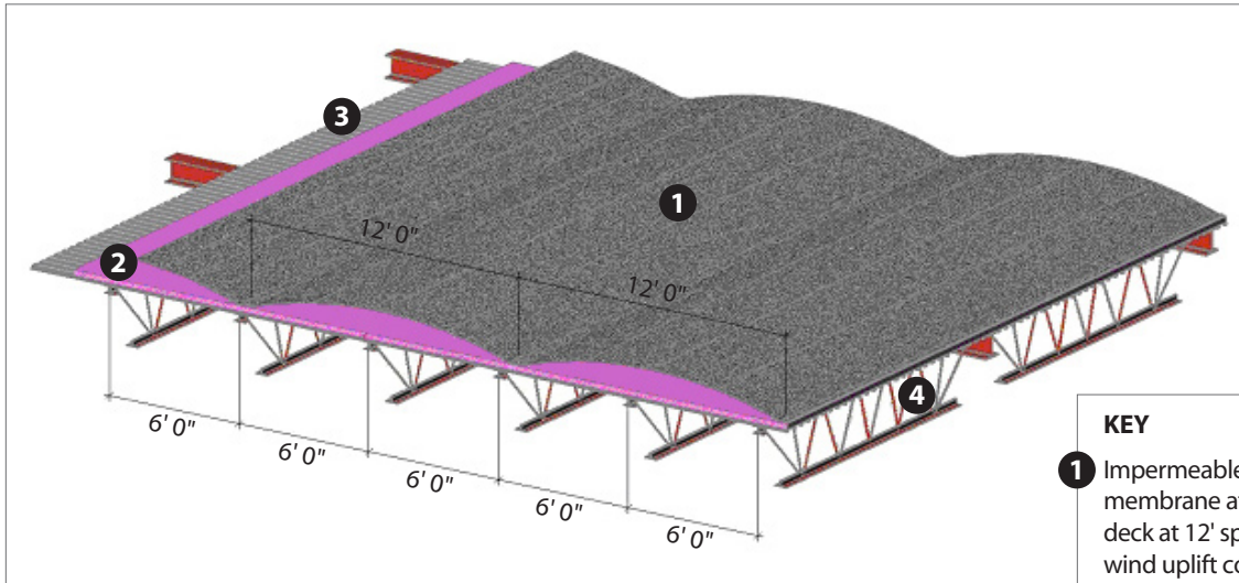
Figure 1 Roofing Membrane Seam Perpendicular to Deck Span
