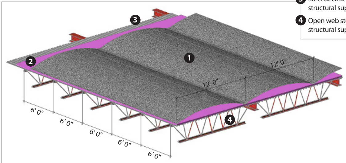
Figure 2 Roofing Membrane Seam Parallel to Deck Span
